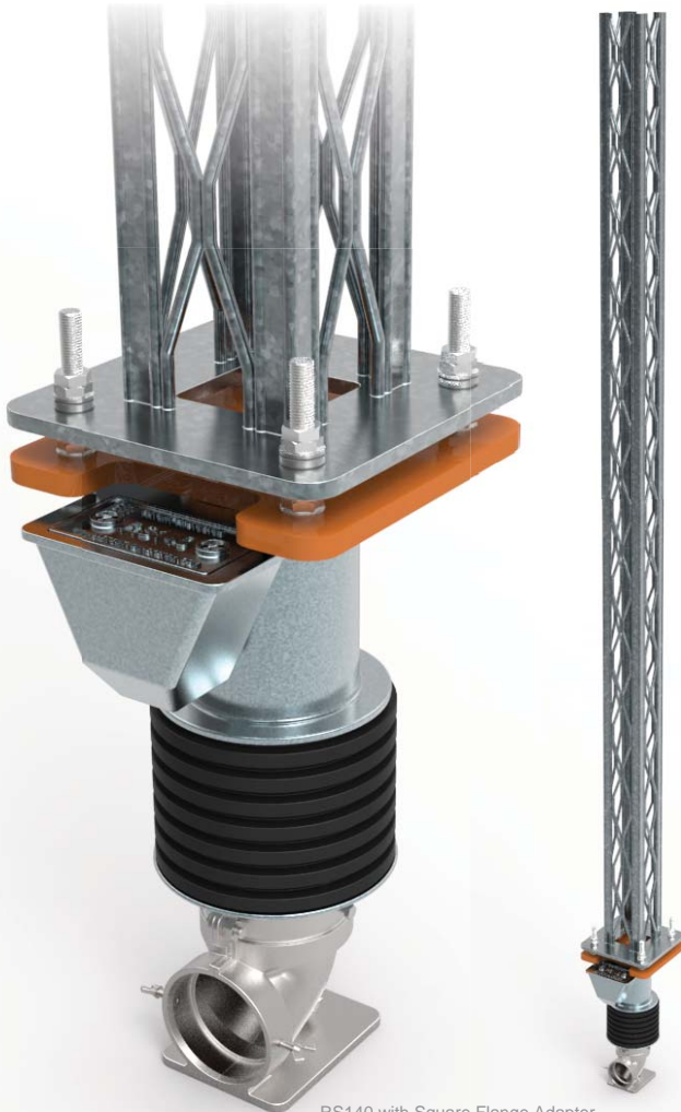
RS140 with Square Flange Adapter
